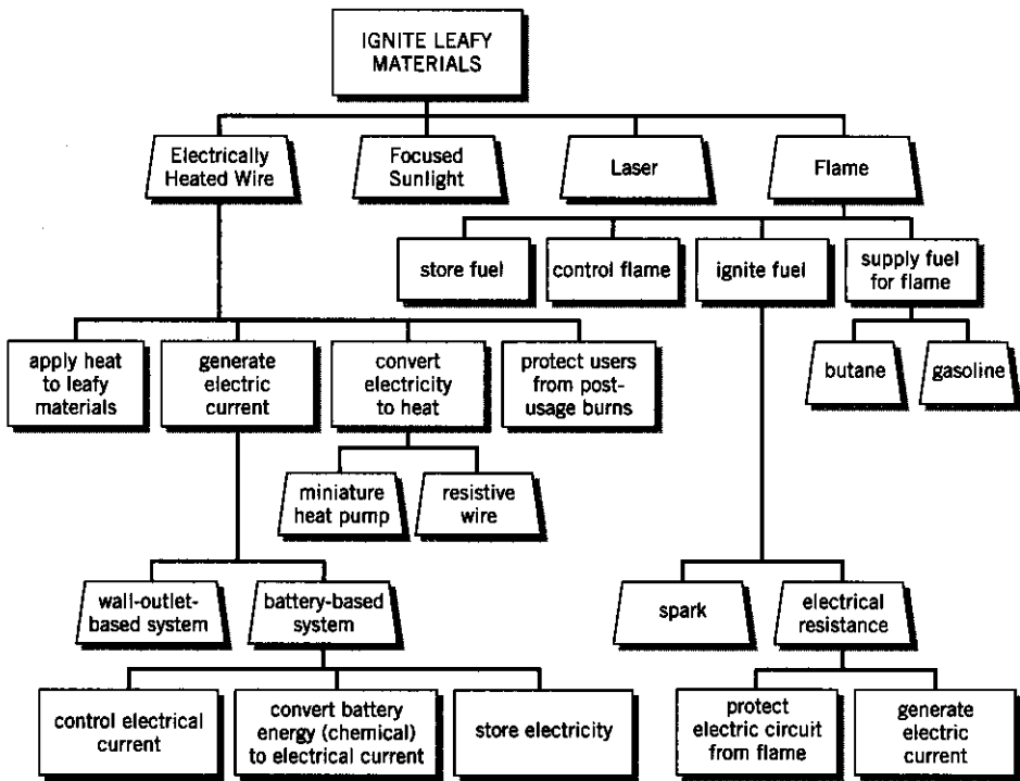
FIGURE 4.2 Part of a function-means tree for a cigarette lighter. (Functions are shown in rectangles, while means are shown in trapezoids.) Notice that there are different subfunctions that result from different means. It is often the case that conceptual design choices will result in very different functions at the preliminary and detailed design stages.
